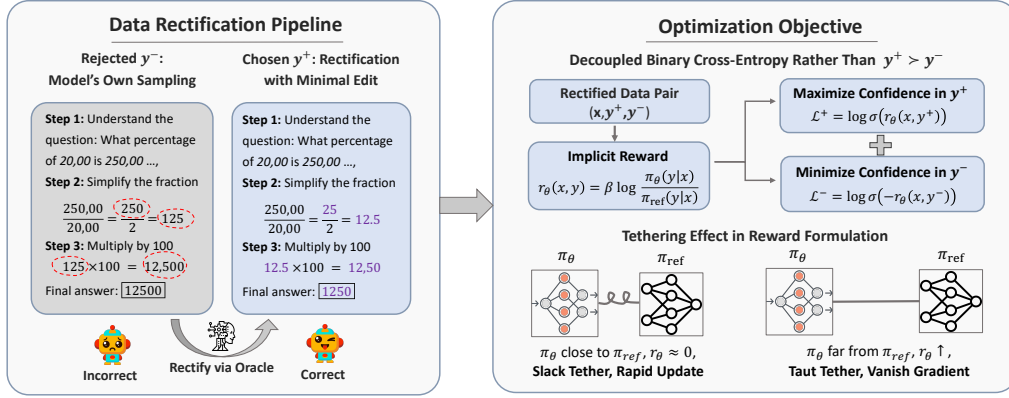
Figure 1: Illustration of SPoT. Left: An Oracle surgically corrects reasoning errors, yielding positive samples proximal to the model’s original distribution. Top-Right: Unlike DPO’s relative ranking, we leverage an explicit classification loss that proves more effective for reasoning tasks. Bottom-Right: The tethering effect inherent in our reward definition substantially mitigates catastrophic forgetting.
