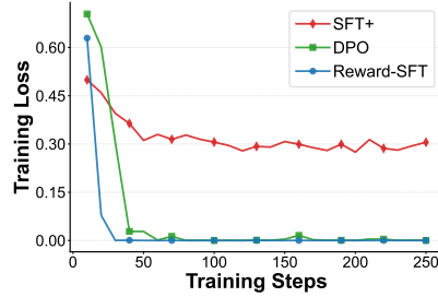
Figure 3: Training loss curve. Reward-SFT and DPO converge rapidly; SFT+ remains high under its negative log-likelihood objective.
