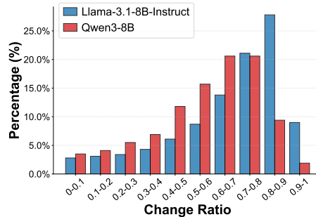
Figure 5: Distributions of change ratio. Higher values indicate less token overlap between the original and rectified responses. The distribution shape is determined by the model ability and the data difficulty together.
