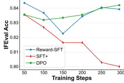
Figure 2: IFEval acc results (avg@5). SFT+ forgets instruction following ability, while reward-based methods do not.
