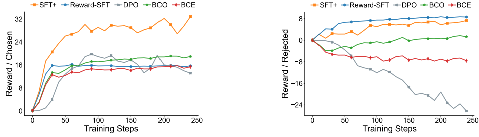
Figure 4: Evolution of implicit rewards during training. Left: reward scores for chosen responses; Right: reward scores for rejected responses. The reward measures how much the model’s preference for the chosen response has grown relative to the initial state.
